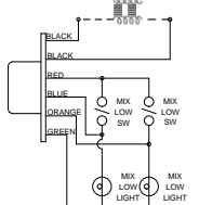
DETAIL "A" MODELS W/"CHIME" OPTION
